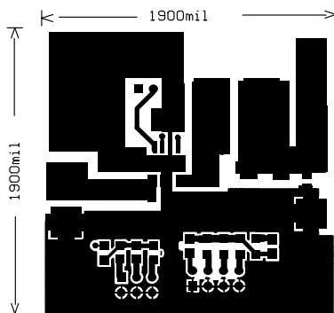
Figure 5c. Top Layer
