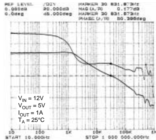
Full-Load Stability Phase Margin = 50°
