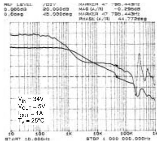
Full-Load Stability Phase Margin = 45°
